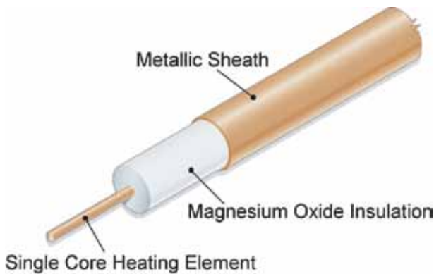
Figure 1. Typical MI cable.
